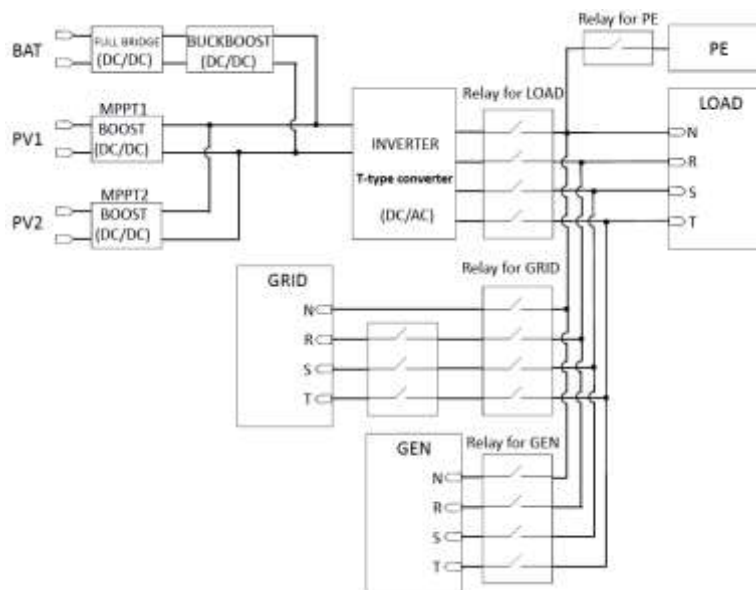
Figure 1 – Block Diagram for model SUN-5K-SG04LP3-EU, SUN-6K-SG04LP3-EU, SUN-8K-SG04LP3-EU, SUN-10K-SG04LP3-EU, SUN-12K-SG04LP3-EU
