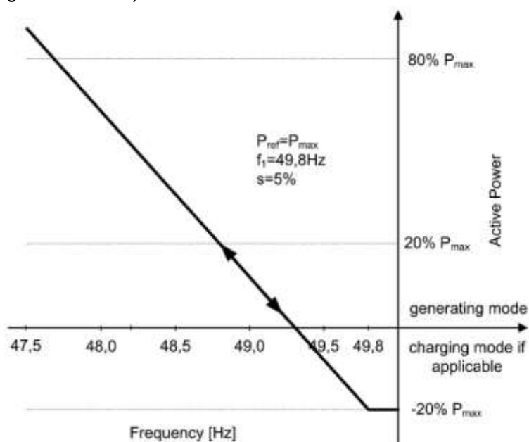
Active power frequency response underfrequency in case of storage device. Example with 20 % power charging at passing of threshold frequency f_1
